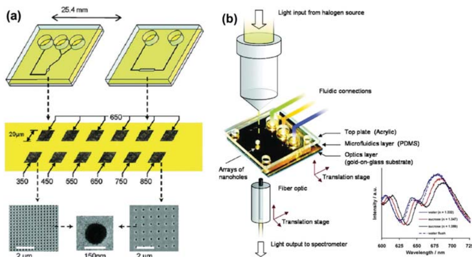
Figure 22. a) Schematic of plasmo-fluidic sensors that integrate microfluidic channels with EOT substrates. b) Schematic of the experimental setup for detection applications. Inset shows the transmission EOT spectra for pure water and sucrose solutions with increasing refractive index. Reproduced with permission. [189] Copyright 2007, American Chemical Society.
