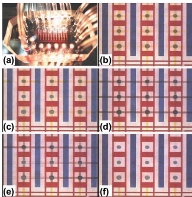
Figure 19. a) Photo of SPR imaging integrated with a microfluidic system. b–f) Consecutive photos of the SPR imaging chip that is carrying out immunoreactions in the microfluidic system. b) Vertical reagent injection step: a reagent (yellow liquid) is injected into the flow channels and then delivered to the Au spots. c) First rinse step: a washing buffer (clear liquid) is injected to rinse the Au spots. d) Horizontal reagent injection step: a reagent (black liquid) is injected into the flow channels then delivered to the Au spots. e) Second rinse step: a washing buffer (clear liquid) is injected to rinse the Au spots. f) The channels in the microfluidic device are clear after the second rinse. Reproduced with permission. [168] Copyright 2008, Royal Society of Chemistry.
