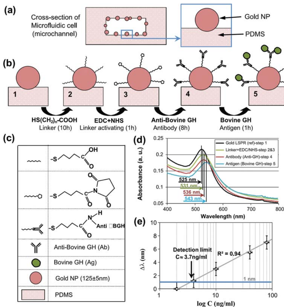
Figure 20. An LSPR-microfluidic sensor based on metal nanoparticles immobilized on the sidewalls of microfluidic channels. a) Cross-sectional view of a microfluidic channel with Au nanoparticles on the sidewalls. b) Schematic illustration of the sensing protocol with legend shown in (c). d) LSPR spectra of Au nanoparticles measured at four different stages. e) Peak shift of LSPRs as a function of analyte concentration. Reproduced with permission. [179] Copyright 2013, Elsevier.
