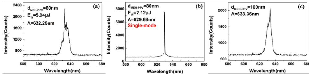
Fig. 6. Lasing emission spectra with different thickness of MEH-PPV films at 14 \mu\text{J/pulse} . (a) For 60 nm thickness film, the peak is at 632 nm and the threshold is 5.94 \mu\text{J/pulse} . (b) For 80 nm thickness film, the peak is at 629 nm and the threshold is 2.12 \mu\text{J/pulse} . The lasing is operated at single-mode. (c) For 100 nm thickness film, the peak is at 633 nm, and no lasing is achieved.
